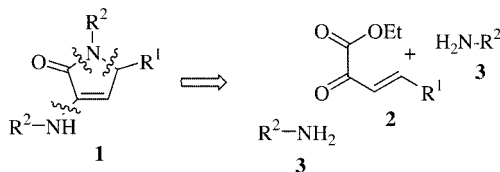
Scheme 1. Retrosynthesis of 3-amino-1,5-dihydro-2H-pyrrol-2-ones ( 1 ).
