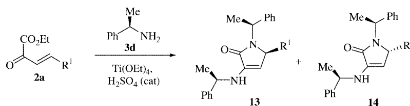
Scheme 5. Synthesis of the optically pure 1,5-dihydro-2 H -pyrrol-2-ones 13 and 14 .
