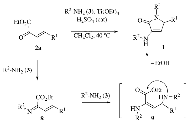
Scheme 3. Synthesis of 1-azadiene 8 and cyclic amines 1 .
