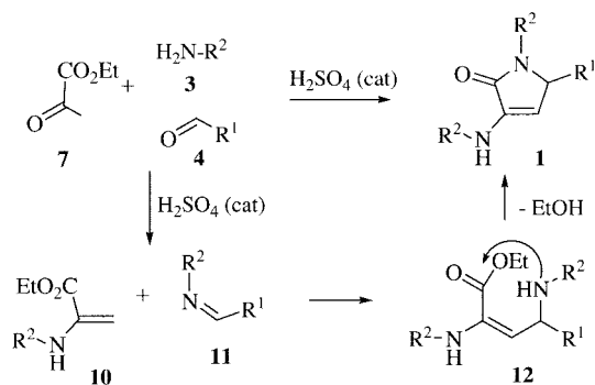
Scheme 4. Proposed mechanism for the three-component reaction.
