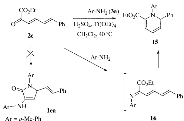
Scheme 6. Synthesis of 1,2-dihydropyridine 15 .
