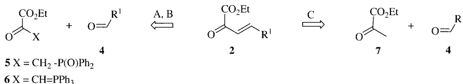
Scheme 2. Synthetic strategies used for the synthesis of \beta,\gamma -unsaturated \alpha -keto esters 2 .
